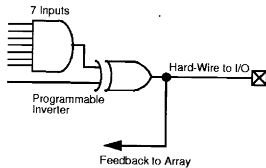
Figure 4• D-Module Implementation
