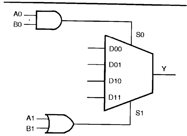
Figure 2• C-Module Implementation
