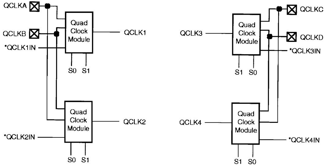
*QCLK1IN, QCLK2IN, QCLK3IN, and QCLK4IN are internally-generated signals.
