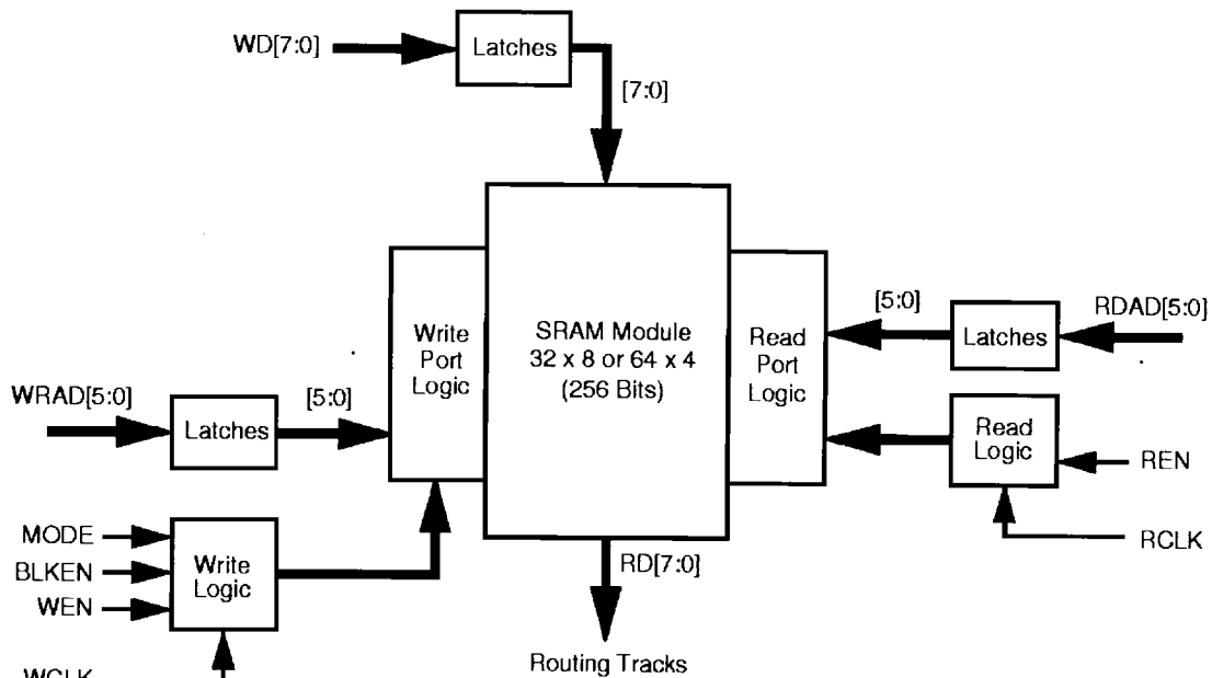
Figure 5• 42MX Dual-Port SRAM Block
