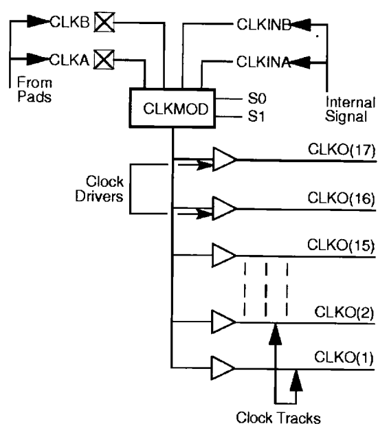
Figure 8• Clock Networks
