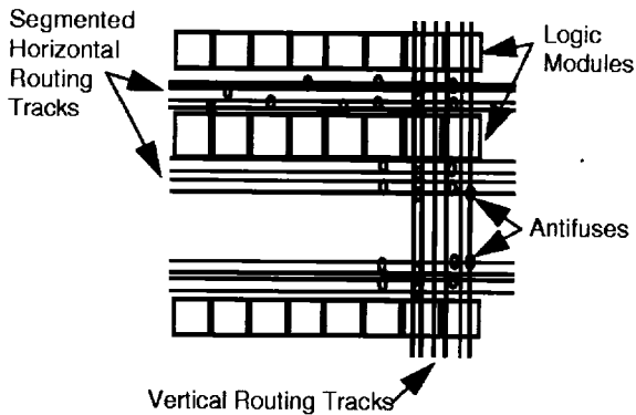
Figure 7• Routing Structure
